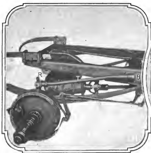
Fig. 11—View of the brakes of the Maxwell Special with the wheel removed showing the jackshaft, torque rod and spring suspension
